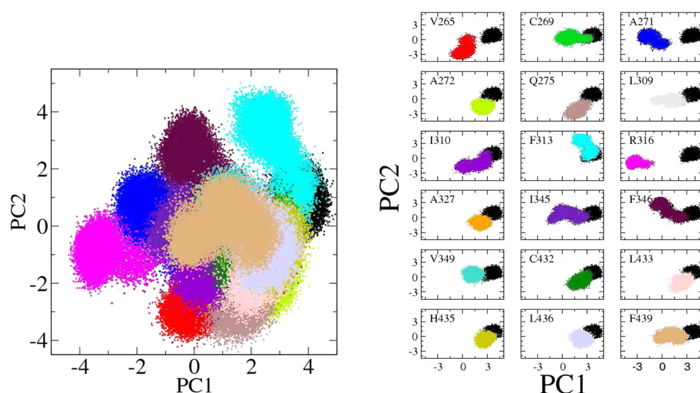
Figure 4. Projection of all snapshots onto top PCs. The configurations of the protein–ligand complex are projected onto PC1 and PC2. Each of the 380000 points represents a specific configuration of the system obtained from a snapshot, as shown at the left. The color scheme matches that of previous figures. Each individual mutant is also displayed in a multipanel view at the right for a clear comparison with the wild type.
