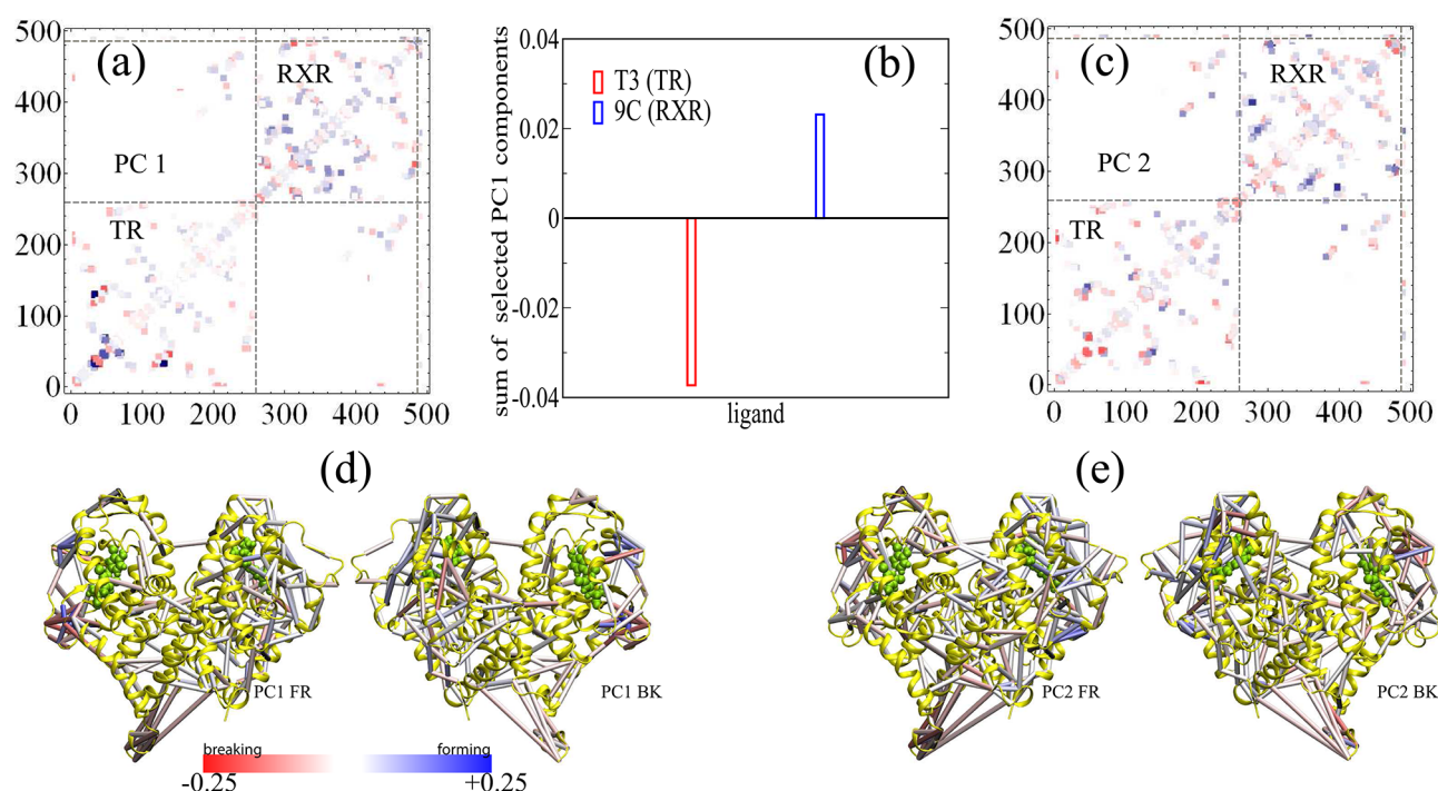
Figure 3. (a) Eigenvector PC1 displayed on the residue–residue contact map. The internal index of the residues is used here for the axes. The dashed lines separate intra- and interprotein contacts. Another set of dashes demarcates the contacts formed between ligands (internal indices 492 and 493) and protein residues. (b) Sum of selected elements in eigenvector PC1 that contain the contact interaction between ligands (T3 and 9C) and the protein complex. The values of individual elements are listed in Figure S4 of the Supporting Information. (c) Eigenvector PC2 displayed on the contact map. Three-dimensional representations of PC1 and PC2 values are shown in panels d and e, respectively. For the sake of clarity, only those contacts with absolute values of >0.03 are explicitly displayed as colored cylinders.
